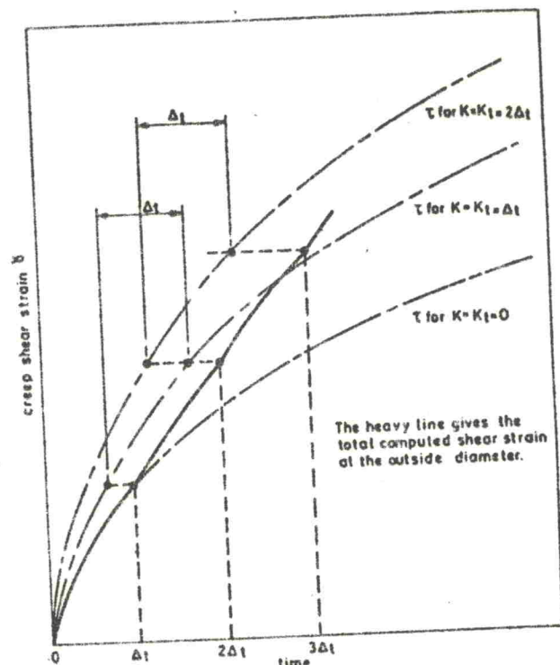
FIG. 2 EXAGGERATED DIAGRAM TO ILLUSTRATE STRAIN-HARDENING METHOD USED TO PREDICT CREEP OF THICK-WALLED CYLINDER
